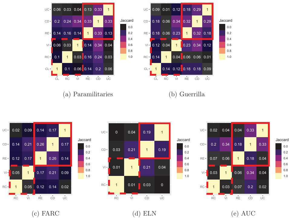
Figure 3. Pairwise Jaccard Similarity.
