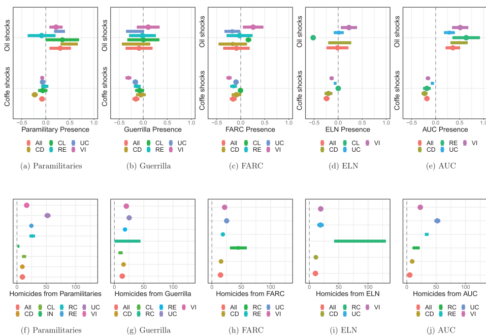
Figure 6. Predicted effects using different measures.
