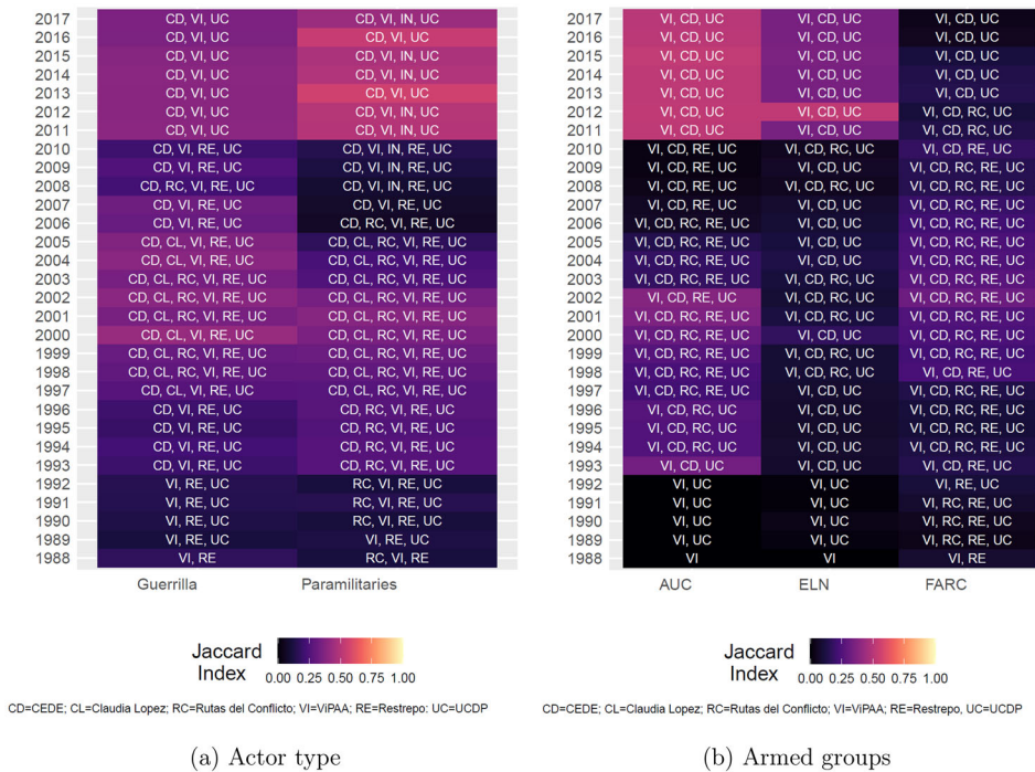
Figure 5. Local Jaccard Similarity.
