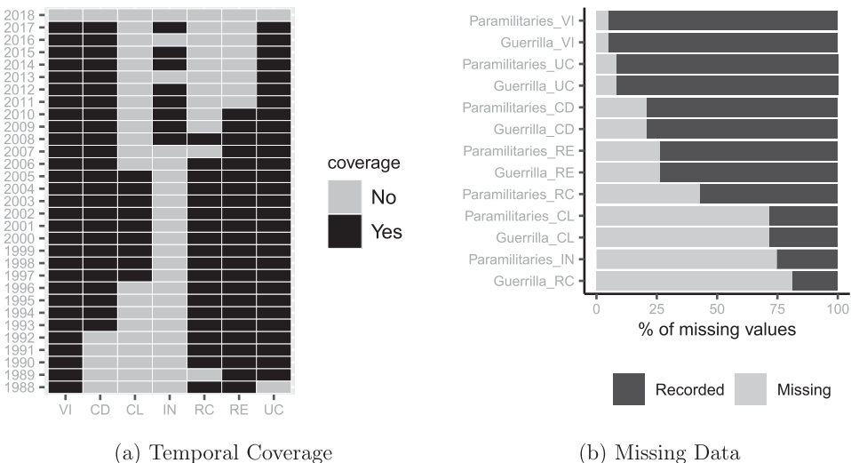
Figure 2. Coverage and missingness.
