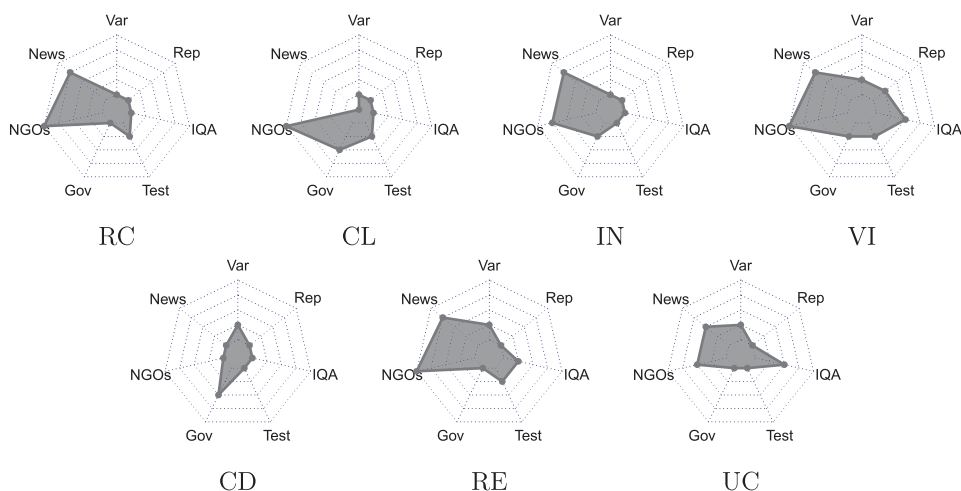
Figure 1. Measurement set characteristics.
