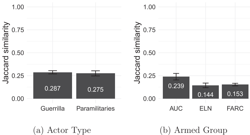
Figure 4. Average Jaccard Similarity.
